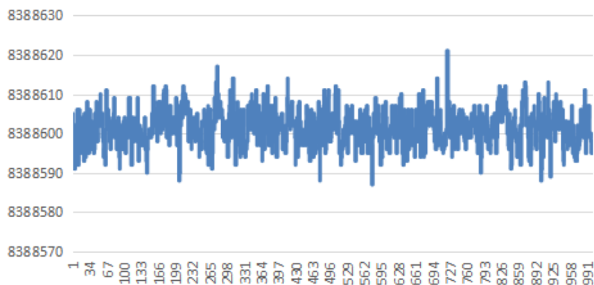
16.7Hz, PGA=1
