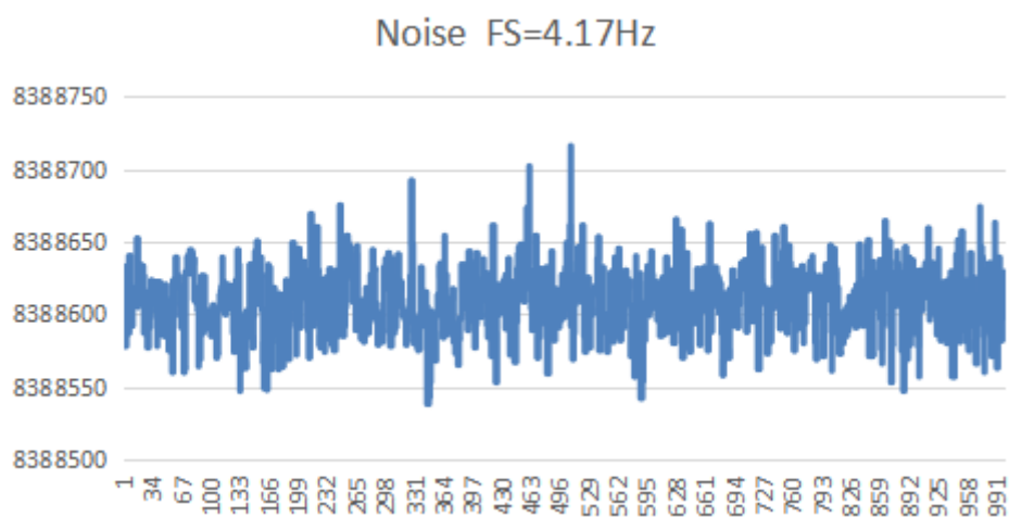
MS5197T 噪声 ( AVDD=4V,VREF = 2.048, Update Rate = 4.17 Hz )
