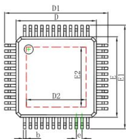
TQFP48/PP (7×7) PACKAGE OUTLINE DIMENSIONS
