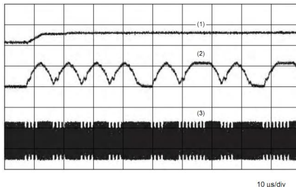
(1) MinLevel (1 V/div) on pin AUX2. (2) Corr1 (1 V/div) on pin AUX1. (3) RF field.
