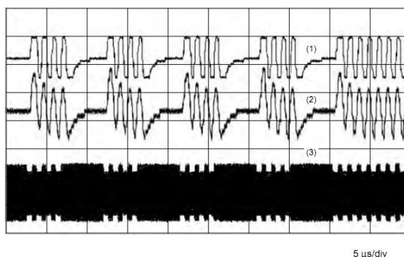
(1) ADC_I (1 V/div) on pin AUX1. (2) ADC_Q (500 mV/div) on pin AUX2. (3) RF field.
