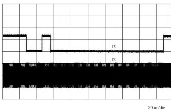
(1) s_data (received data stream) (2 V/div). (2) RF field.
