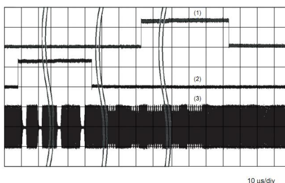
(1) RxActive (2 V/div) on pin AUX1. (2) TxActive (2 V/div) on pin AUX2. (3) RF field.
